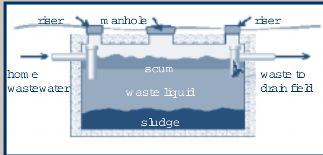
Septic Tank
